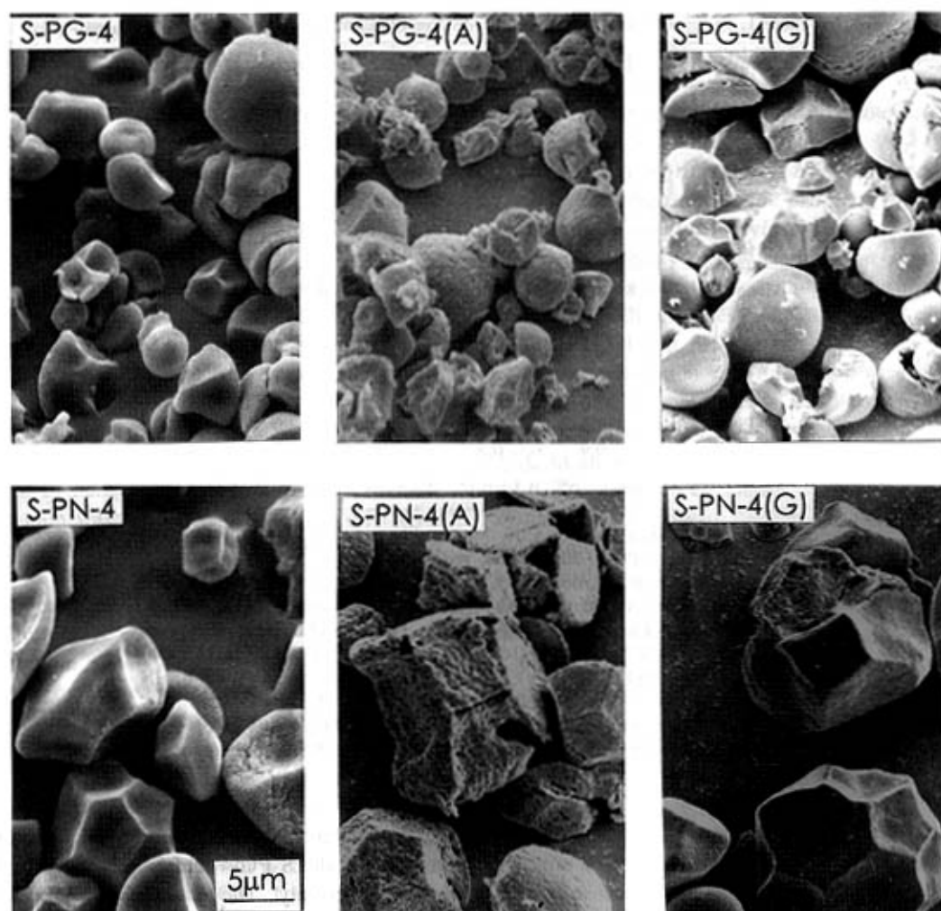
Fig. 2. Scanning electron micrographs of PG-4 and PN-4 starches and their starches digested by \alpha -amylase or glucoamylase for 1 h.
