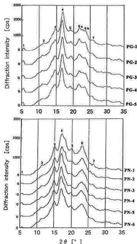
Fig. 3. X-ray diffractograms of PG and PN starches.
